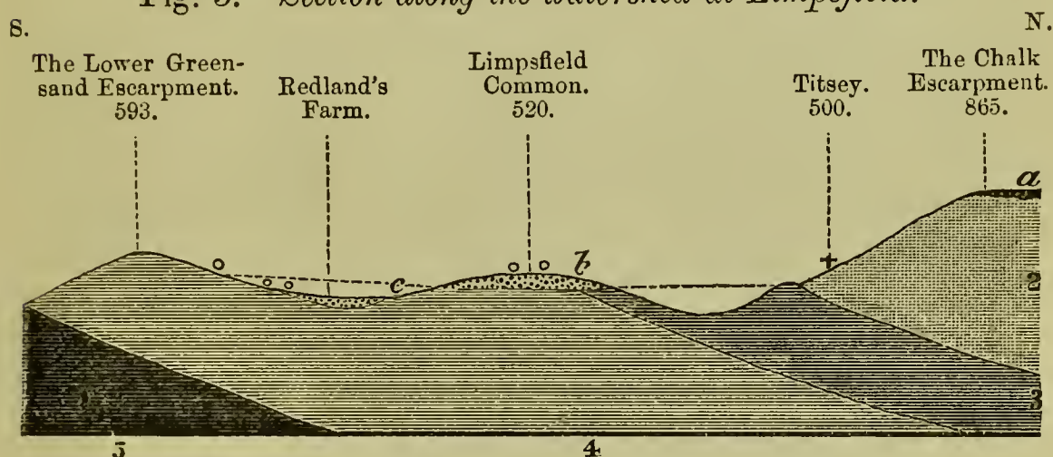
Fig. 5.—Section along the watershed at Limpsfield.
